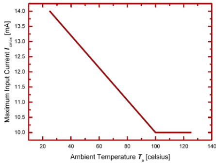
Figure 1. Maximum input current I_{cmax} -Ambient Temperature T_a
