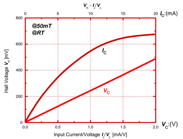
Figure 5. Hall voltage V_H as a function of electrical stimuli I_e/V_C .
