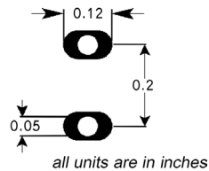
TO-220-2
