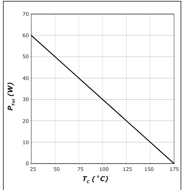
Figure 4. Power Derating
