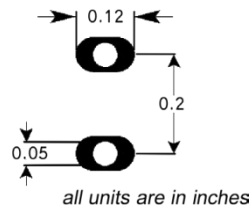
TO-220-2
