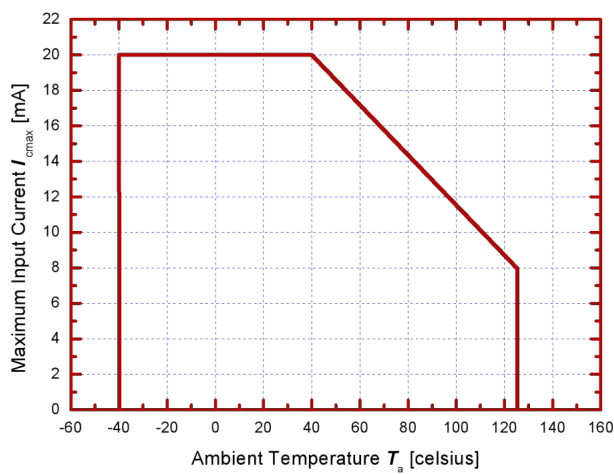
Figure 1.1 Maximum input current I_{cmax}
